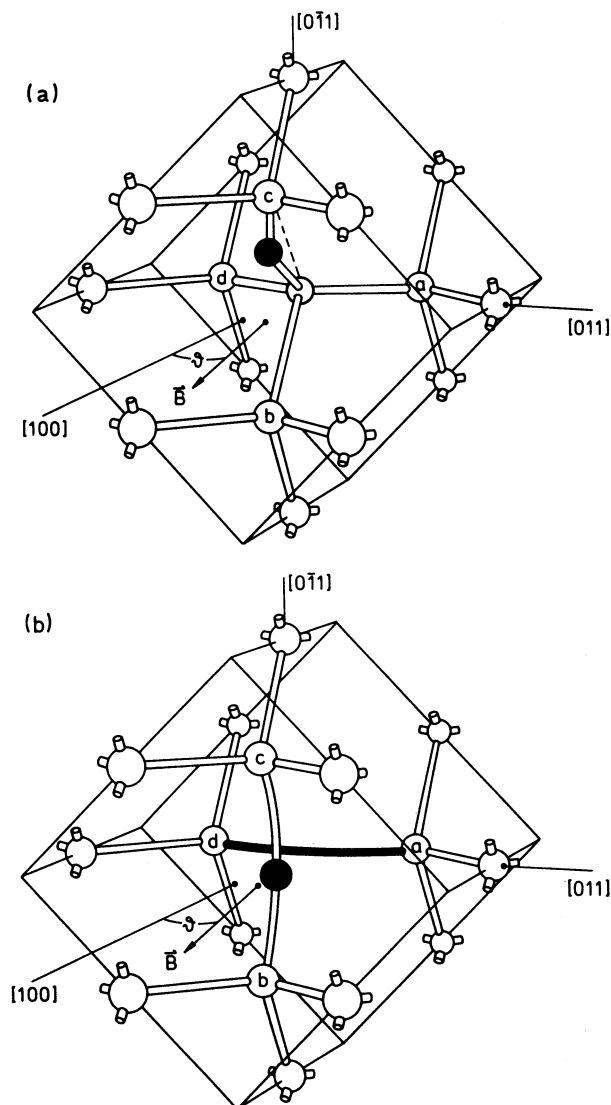
FIG. 1. Model of oxygen (solid sphere) in silicon, (a) before and (b) after electron irradiation. The oxygen-vacancy complex in (b) is shown in orientation ad , in which the defect electron is mainly localized in the reconstructed bond between the atoms a and d . All further data refer to this standard orientation ad .
