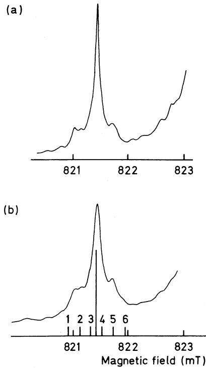
FIG. 3. EPR spectrum of \text{O-V}^- for orientation bc with \mathbf{B} \parallel [011] . (a) For a sample with natural oxygen; (b) for a sample enriched to about 40% in ^{17}\text{O} . Calculated positions and relative intensities of the ^{17}\text{O} hyperfine lines are indicated. Numbers refer to EPR transitions which belong to the following nuclear-spin states: 1, m_I = +\frac{5}{2} ; 2, m_I = +\frac{3}{2} ; 3, m_I = +\frac{1}{2} ; 4, m_I = -\frac{1}{2} ; 5, m_I = -\frac{3}{2} ; 6, m_I = -\frac{5}{2} . The relative intensity change between the two ^{29}\text{Si} hyperfine satellites at the left of the central line is just visible.
