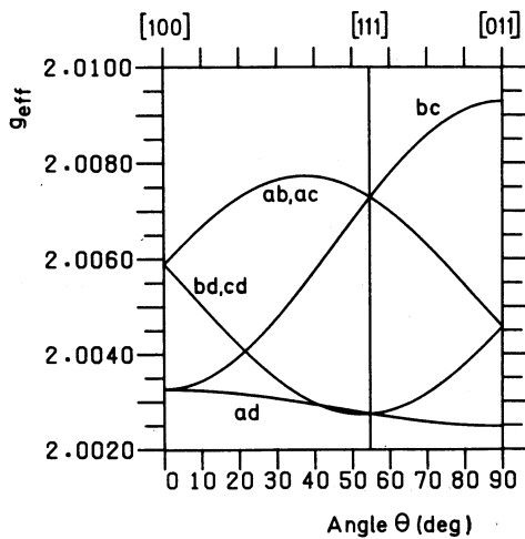
FIG. 2. Angular dependence of the effective g values, g_{\text{eff}} , of the Si-B1 EPR spectrum for the magnetic field rotating in the (0 \bar{1} 1) plane. The labels of the orientations correspond to Fig. 1(b).
