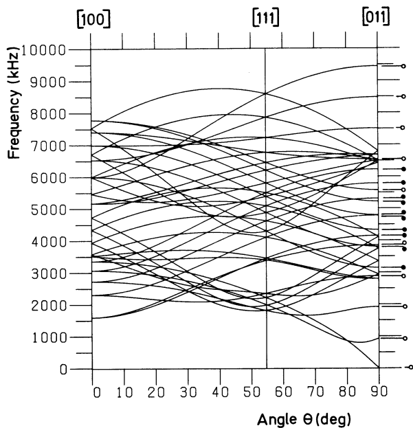
FIG. 4. Angular dependence of the ENDOR frequencies for rotation of the magnetic field \mathbf{B} in the (0\bar{1}1) plane. The frequencies found for the EPR orientations bc and ad are indicated: ○ denotes orientation bc and ● denotes orientation ad . Note that the frequency scale is absolute. The microwave frequency was 22.9713 GHz.
